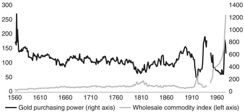
Figure 8 Purchasing power of gold and wholesale commodity index in England, 1560–1976.
